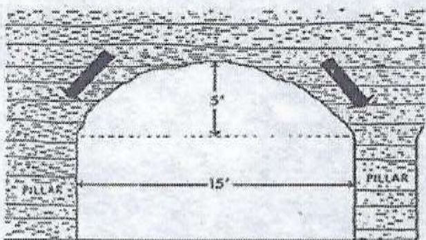
4. Roof has fallen completely and forces are transmitted to pillars. Falling may take minutes, days or even months.
